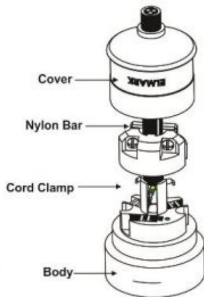
Fig 3. Assembly Diagram
